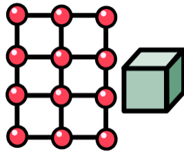
solid
