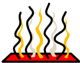
heating
