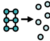
change state
