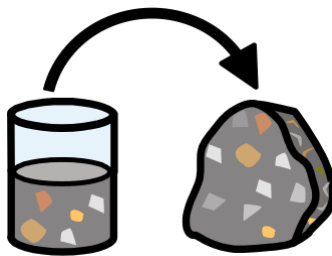
solidification
