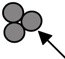
molecules
