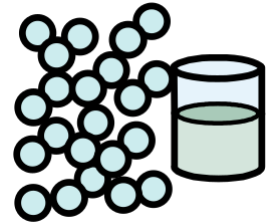
liquid
